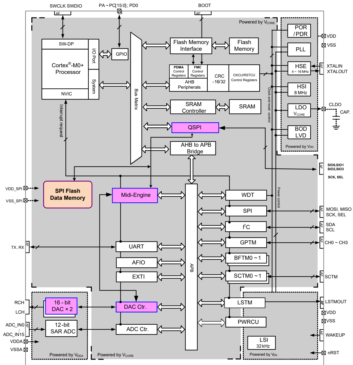
Figure 1. Block Diagram
