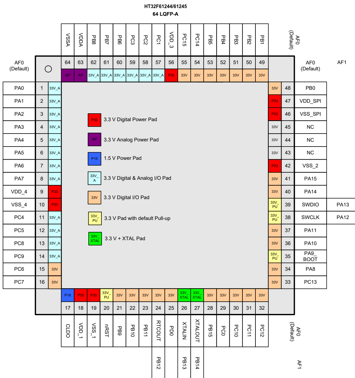
Figure 5. 64-pin LQFP Pin Assignment
