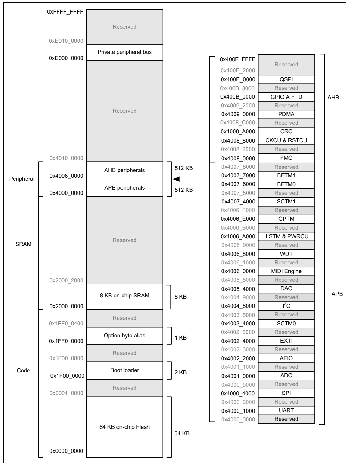
Figure 2. Memory Map
