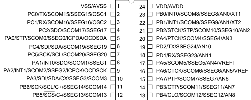
HT66F3195/HT66V3195 24 SSOP-A
