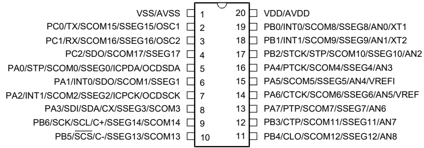
HT66F3195/HT66V3195 20 NSOP-A
