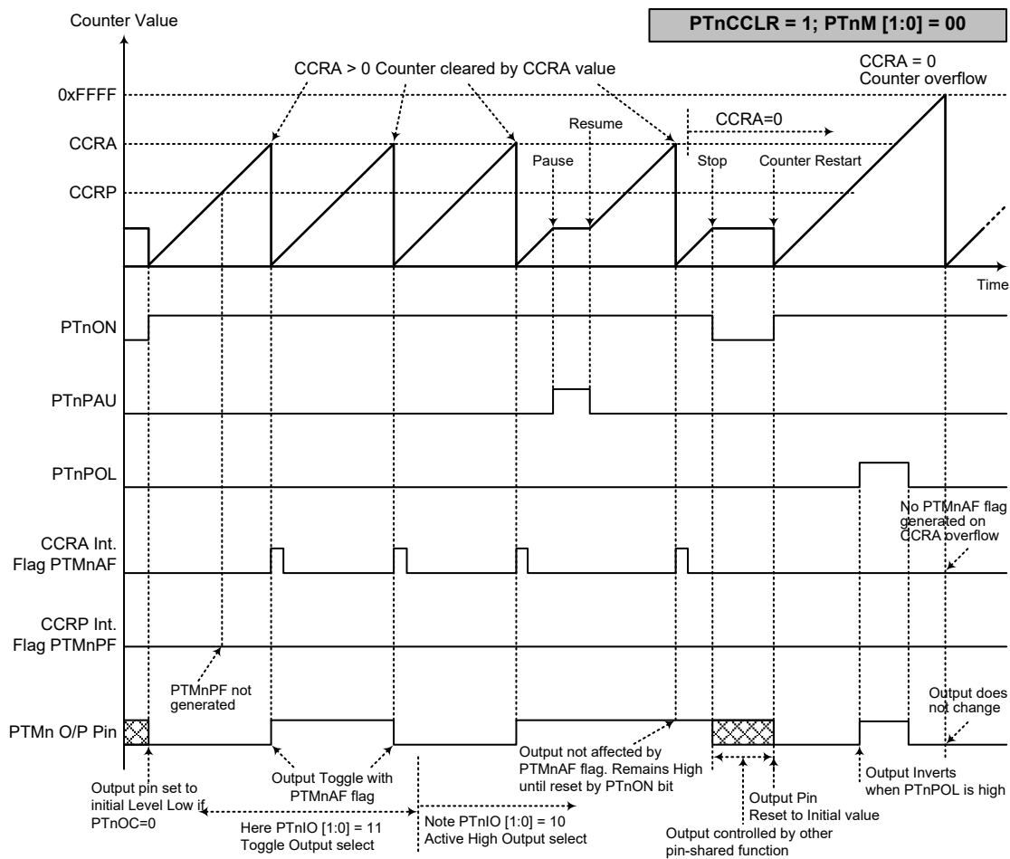
Compare Match Output Mode – PTCCLR=1 (n=0~1)
