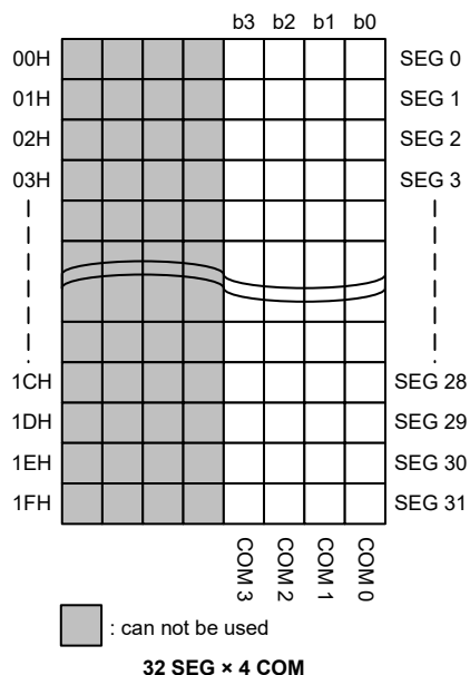
32 SEG × 4 COM LCD Memory Map – HT67L2550A
