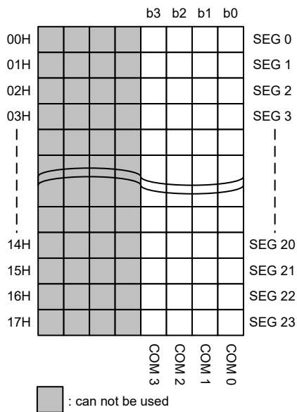
24 SEG × 4 COM LCD Memory Map – HT67L2540A
