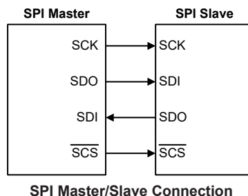
SPI Master/Slave Connection
