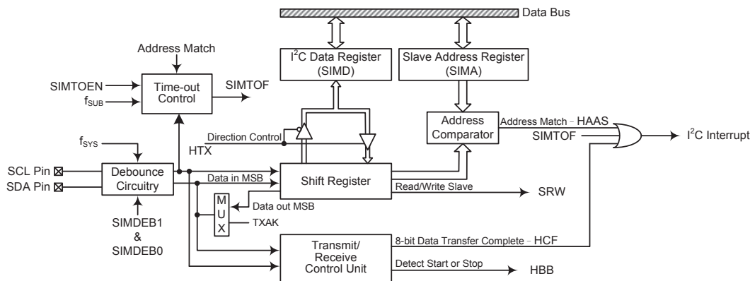
I 2 C Block Diagram
