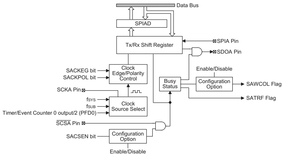
SPIA Block Diagram
