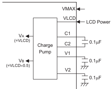
C type 1/2 Bias -- V A = LCD Power V A : LCD Operating Voltage
