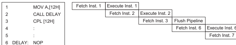
Instruction Fetching
