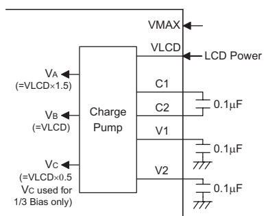
C type 1/3 Bias -- V A = 1.5 x LCD Power V A : LCD Operating Voltage
