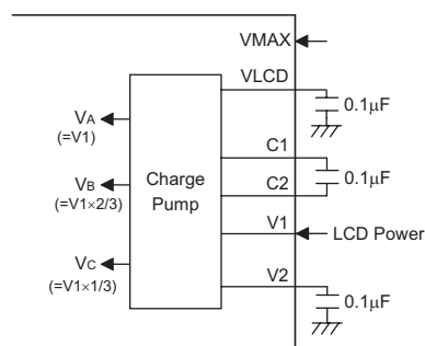
C type 1/3 Bias -- V A = LCD Power V A : LCD Operating Voltage
