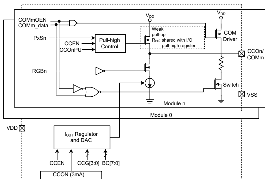
Constant Current LED Driver Block Diagram (CCO & COM)
