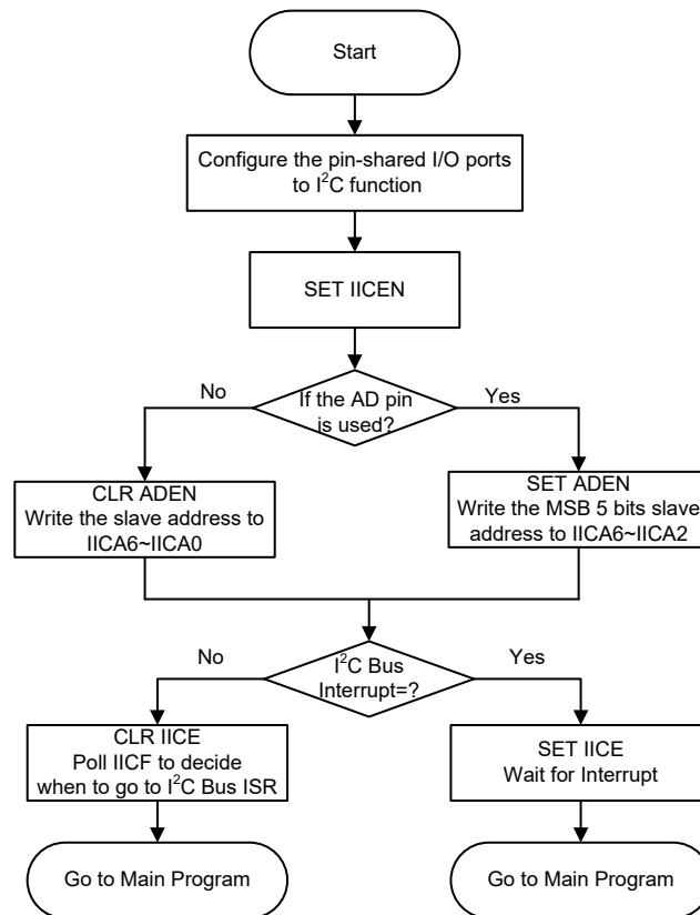
I²C Bus Initialisation Flow Chart
