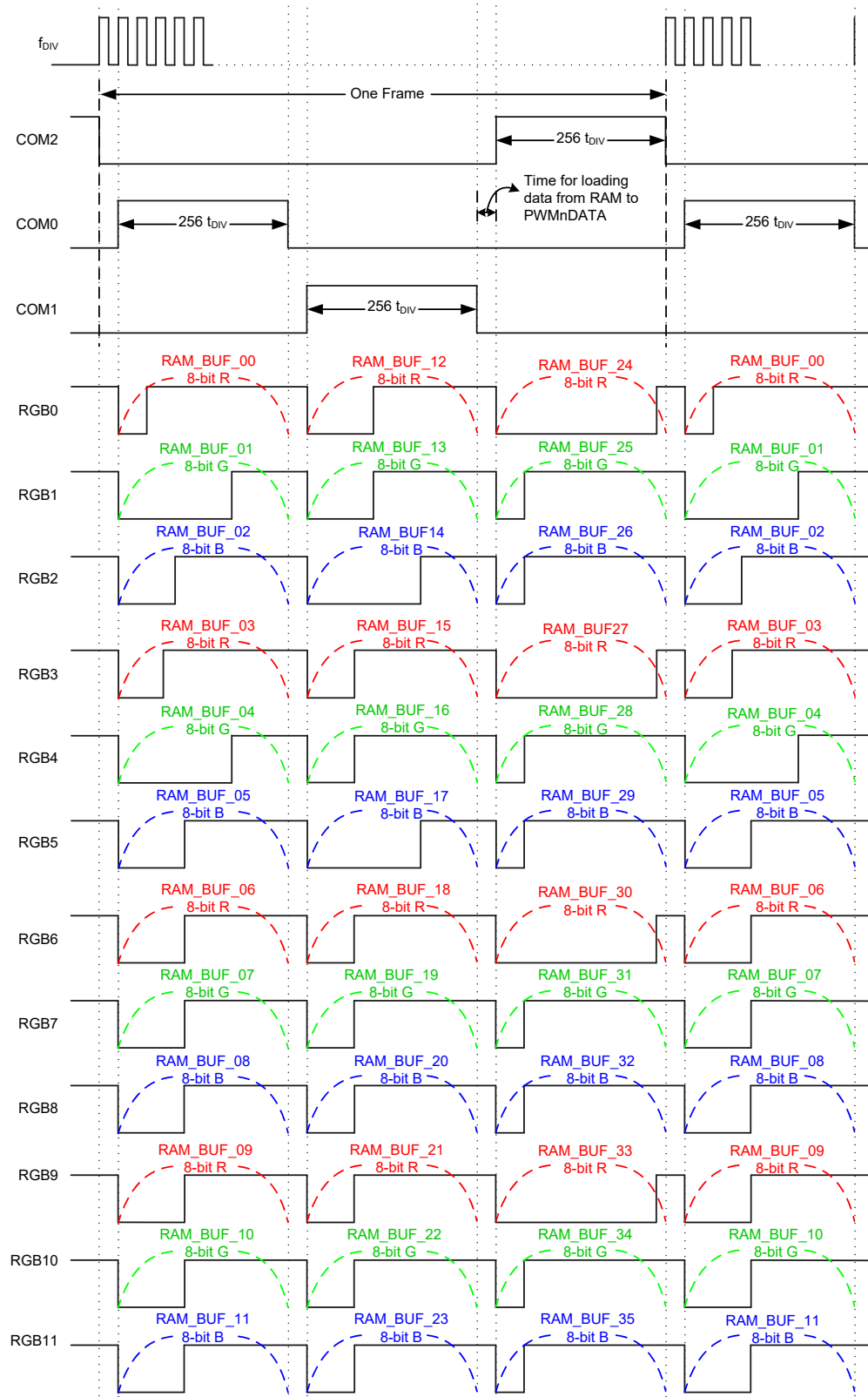
LED PWM Timing for Time-shared Scanning Mode – 3×COM
