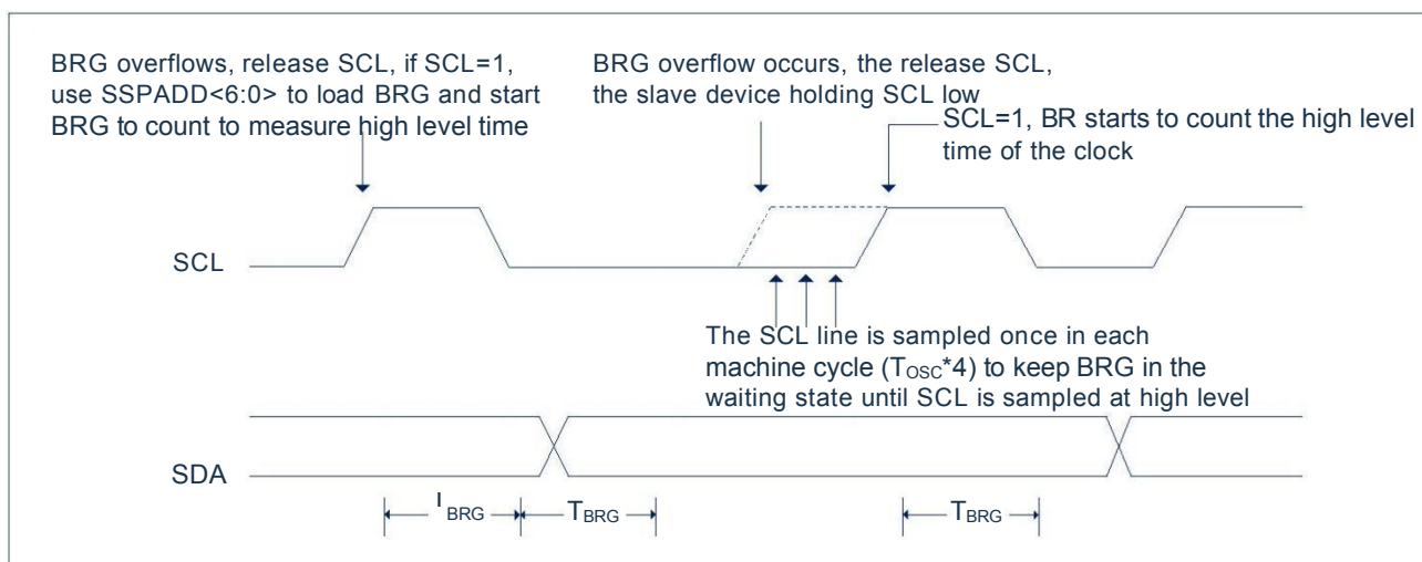
Fig 15-16: clock arbitration in master control transmit mode
