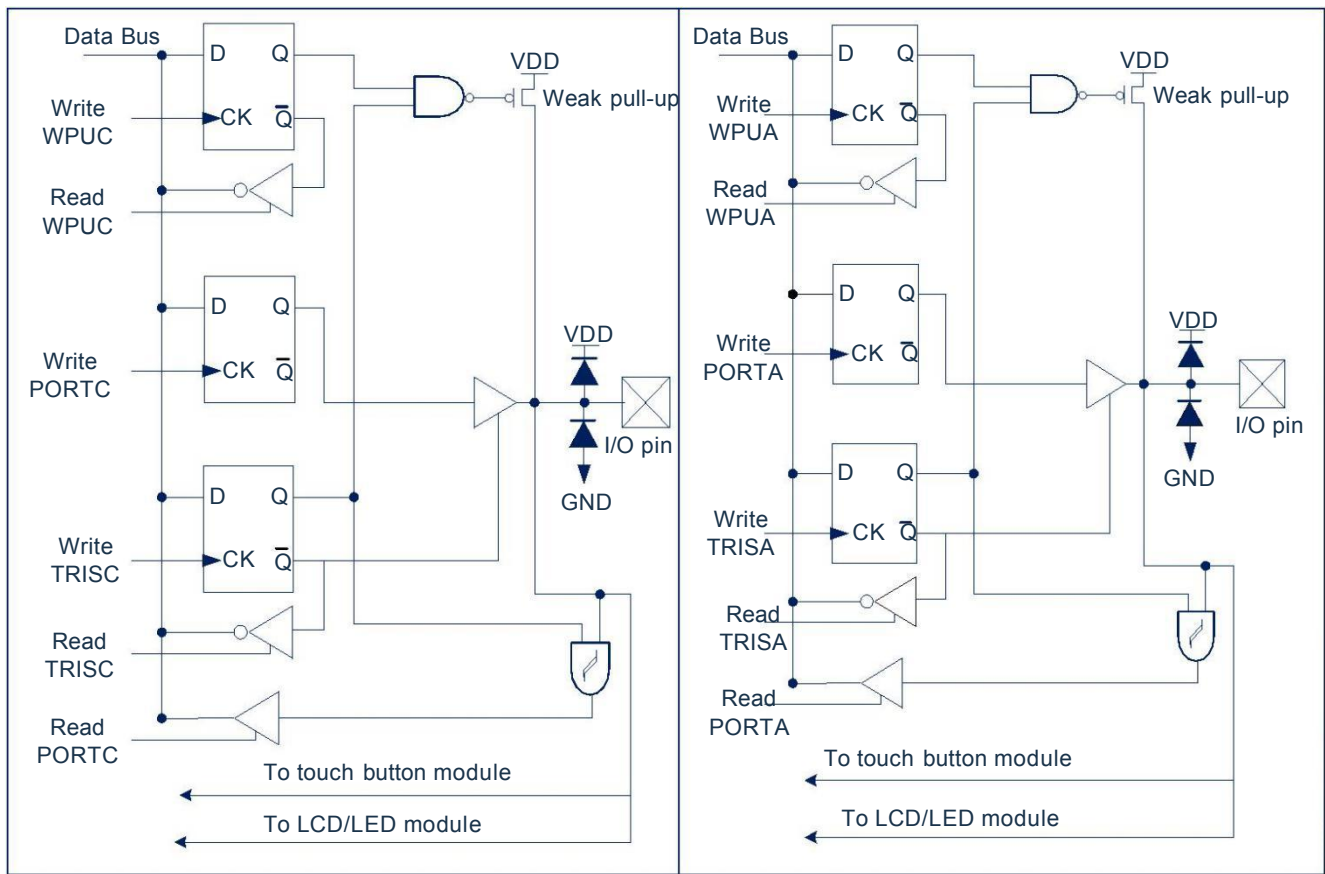
Fig 6-1: I/Oport structure (1)
