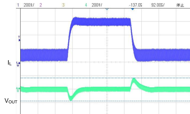
(16) Load Transient(VIN=50.0V,VOUT=12V,IOUT=0.1→0.6A)
