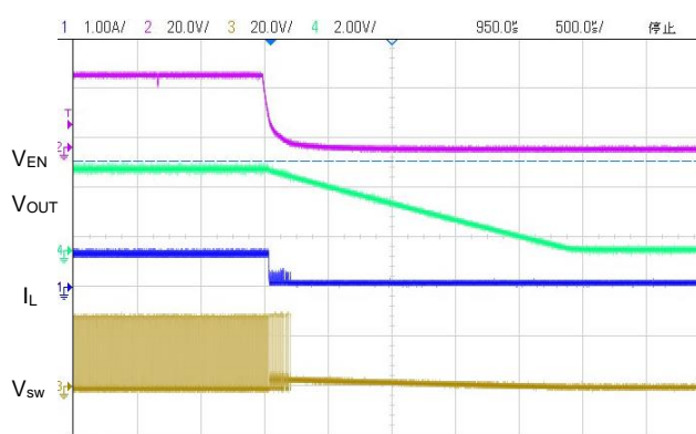
(18) Enable Shutdown(VIN=30.0V,VOUT=3.3V,IOUT=0.6A)
