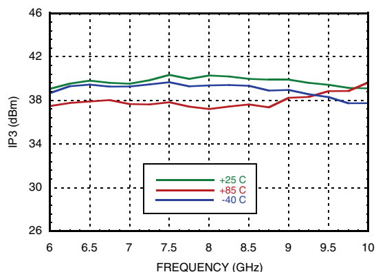
Output IP3 vs. Temperature 7V @ 520 mA, Pin/Tone = -15 dBm
