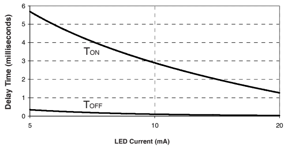
Figure 8. Typical Delay Times
