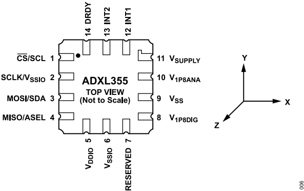
Figure 7. ADXL355 Pin Configuration
