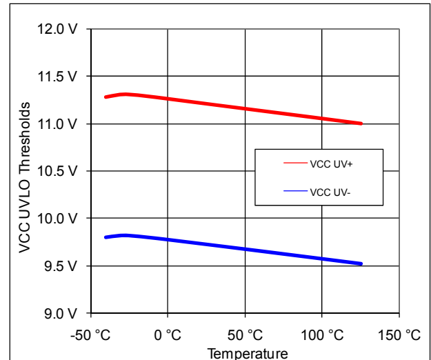
Figure 2: Undervoltage Lockout vs. Temperature
