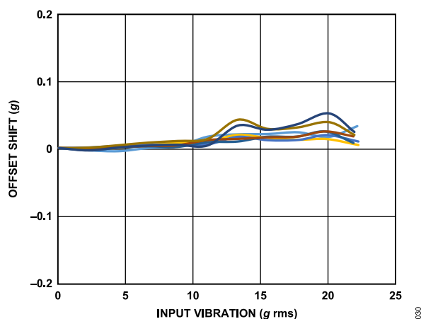
Figure 27. VRE, Y-Axis Offset from -1 g, \pm 40 g Range, Y-Axis Orientation = -1 g
