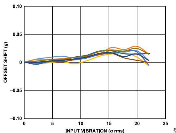
Figure 26. VRE, X-Axis Offset from -1 g, \pm 40 g Range, X-Axis Orientation = -1 g
