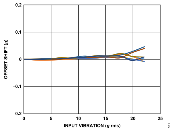
Figure 28. VRE, Z-Axis Offset from -1 g, \pm 40 g Range, Z-Axis Orientation = -1 g
