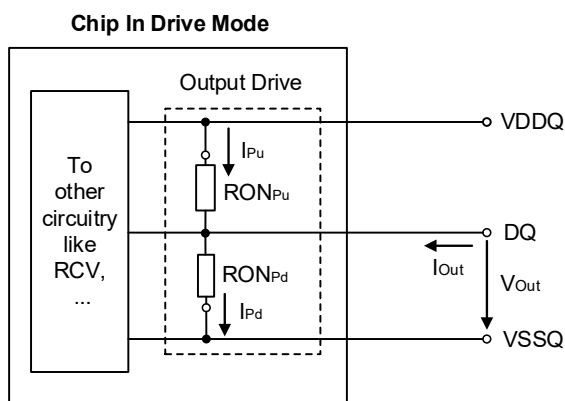
Figure 6-6. Output Driver: Definition of Voltages and Currents
