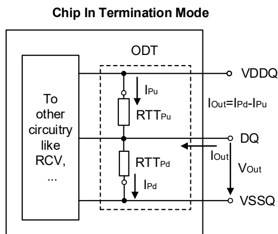
Figure 6-7. On-Die Termination: Definition of Voltages and Currents
