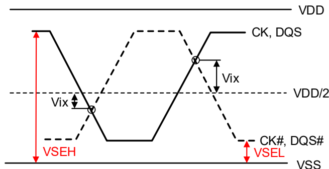
Figure 5-4. V_{ix} Definition
