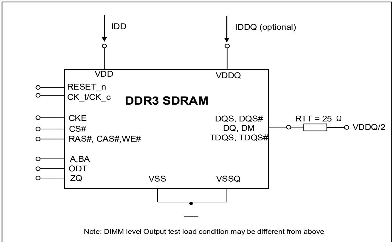
Figure 7-1. Measurement Setup and Test Load for I_{DD} and I_{DDQ} (optional) Measurements
