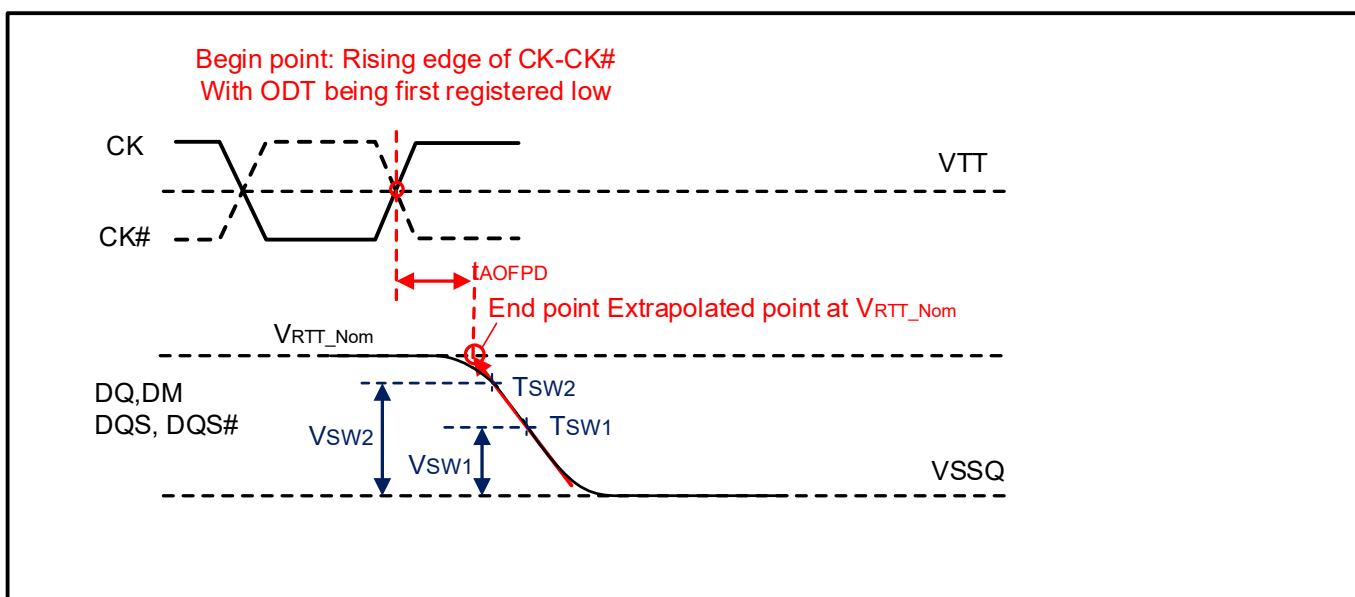
Figure 6-12. Definition of t_{AOFPD}
