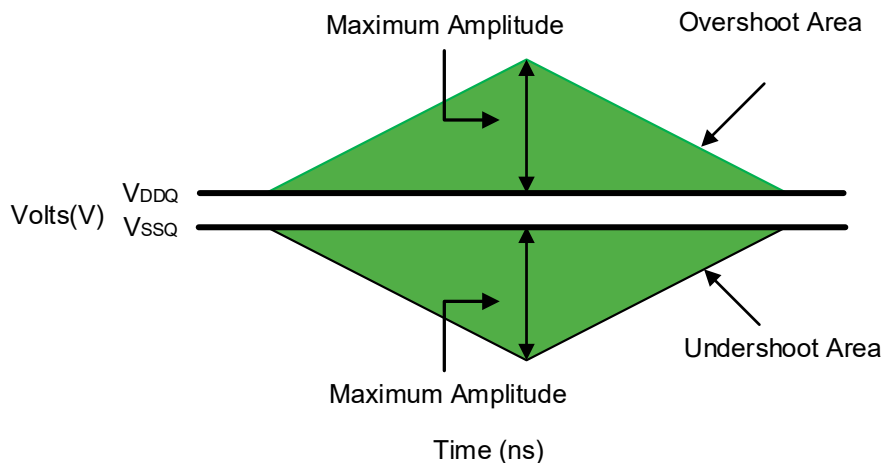
Figure 6-5. Clock, Data, Strobe and Mask Overshoot and Undershoot Definition
