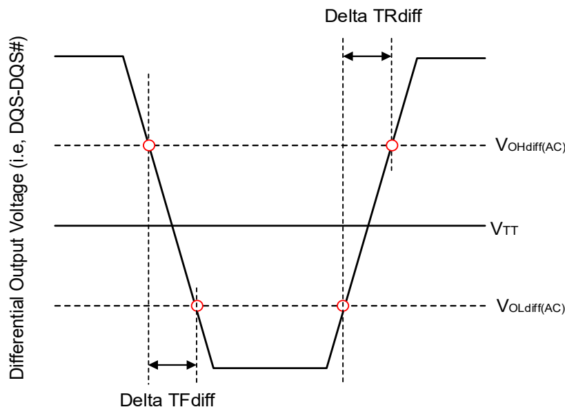
Figure 6-2. Differential Output Slew Rate Definition
