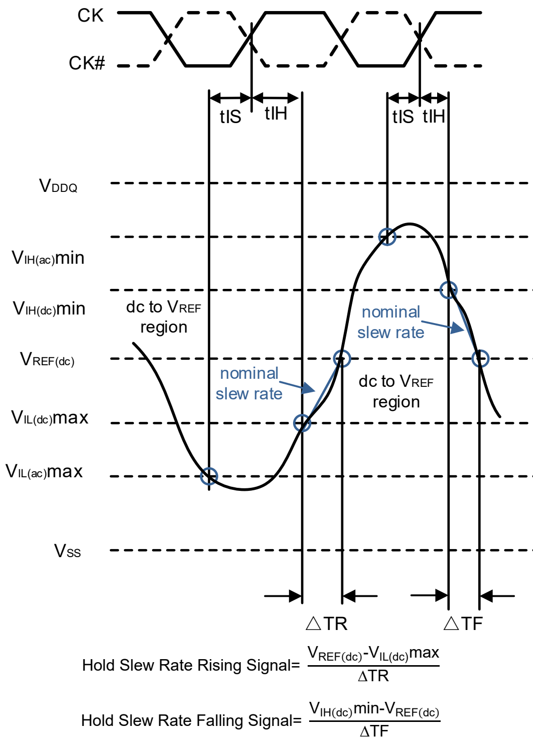
Figure 10-2. Illustration of nominal slew rate for hold time t_{IH} (for ADD/CMD with respect to clock).
