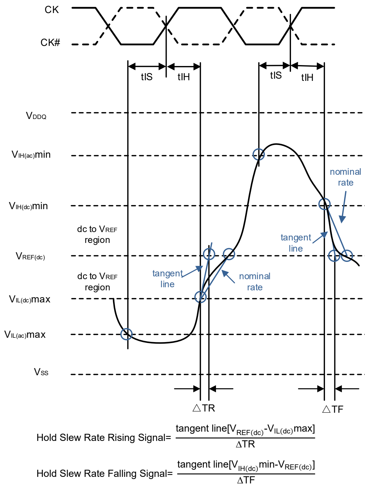
Figure 10-4. Illustration of tangent line for hold time t_{\text{IH}} (for ADD/CMD with respect to clock).
