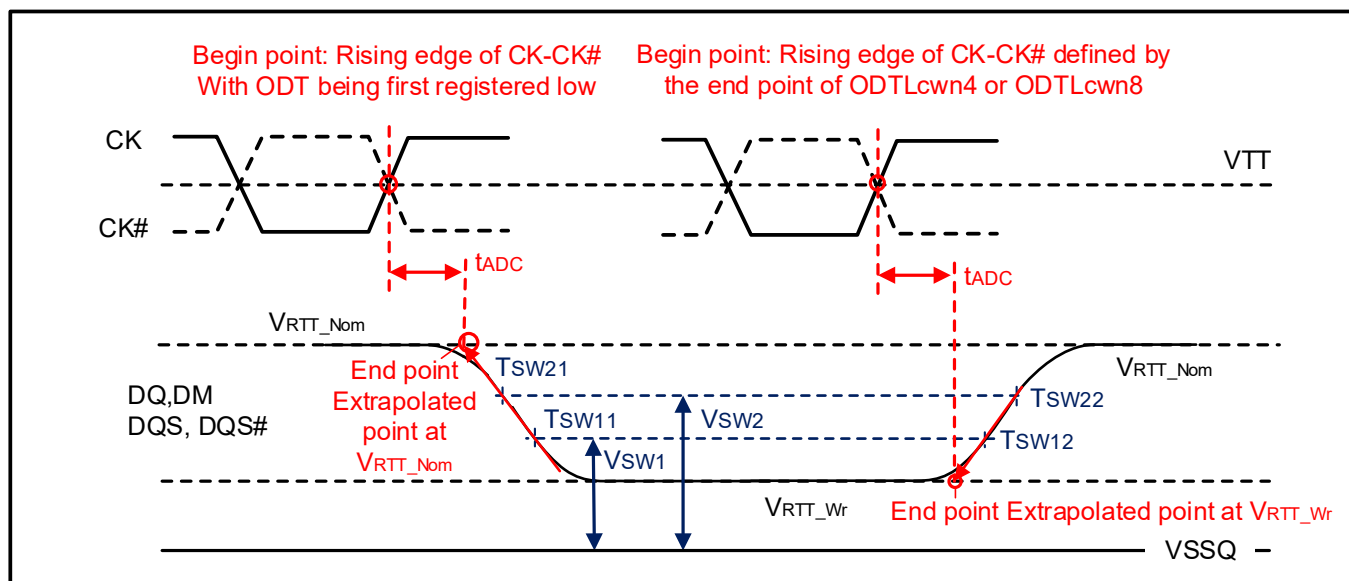
Figure 6-13. Definition of t_{ADC}
