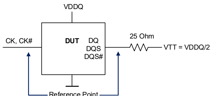
Figure 6-3. Reference Load for AC Timing and Output Slew Rate
