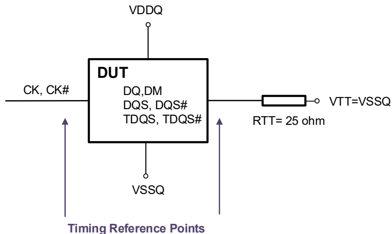
Figure 6-8. ODT Timing Reference Load
