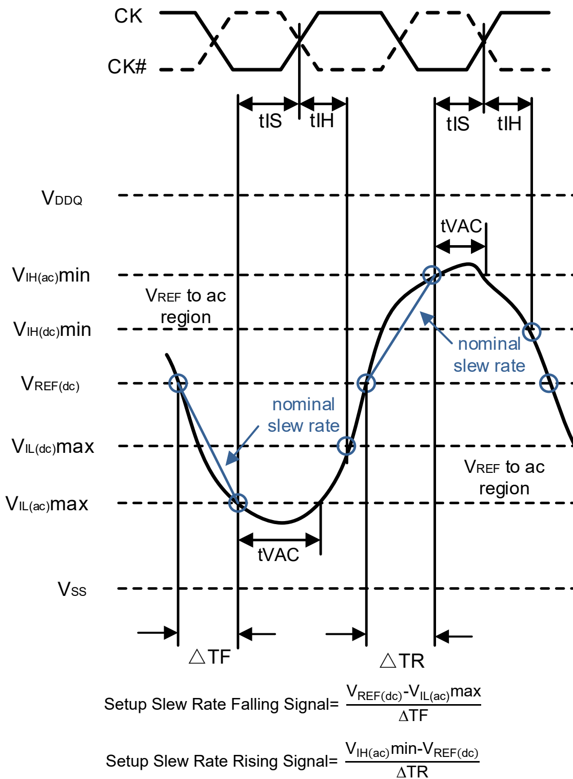
Figure 10-1. Illustration of nominal slew rate and t_{VAC} for setup time t_{IS} (for ADD/CMD with respect to clock).
