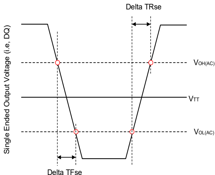
Figure 6-1. Single-ended Output Slew Rate Definition
