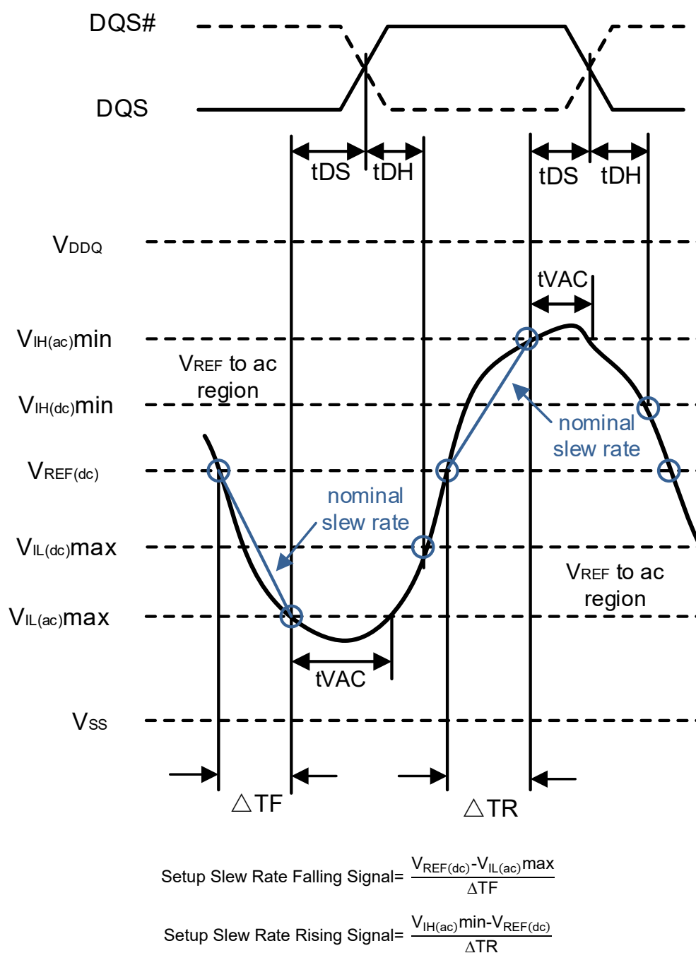
Figure 10-5. Illustration of nominal slew rate and t_{VAC} for setup time t_{DS} (for DQ with respect to strobe)
