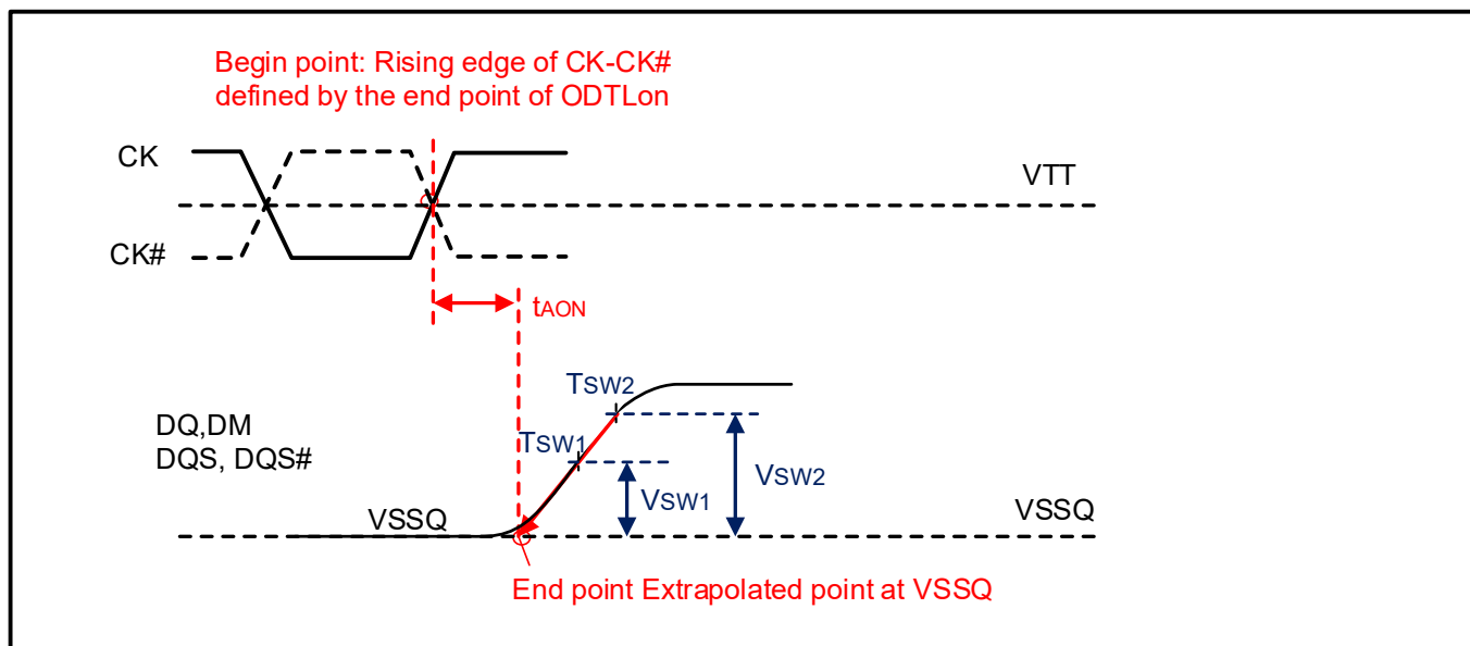
Figure 6-9. Definition of t_{AON}
