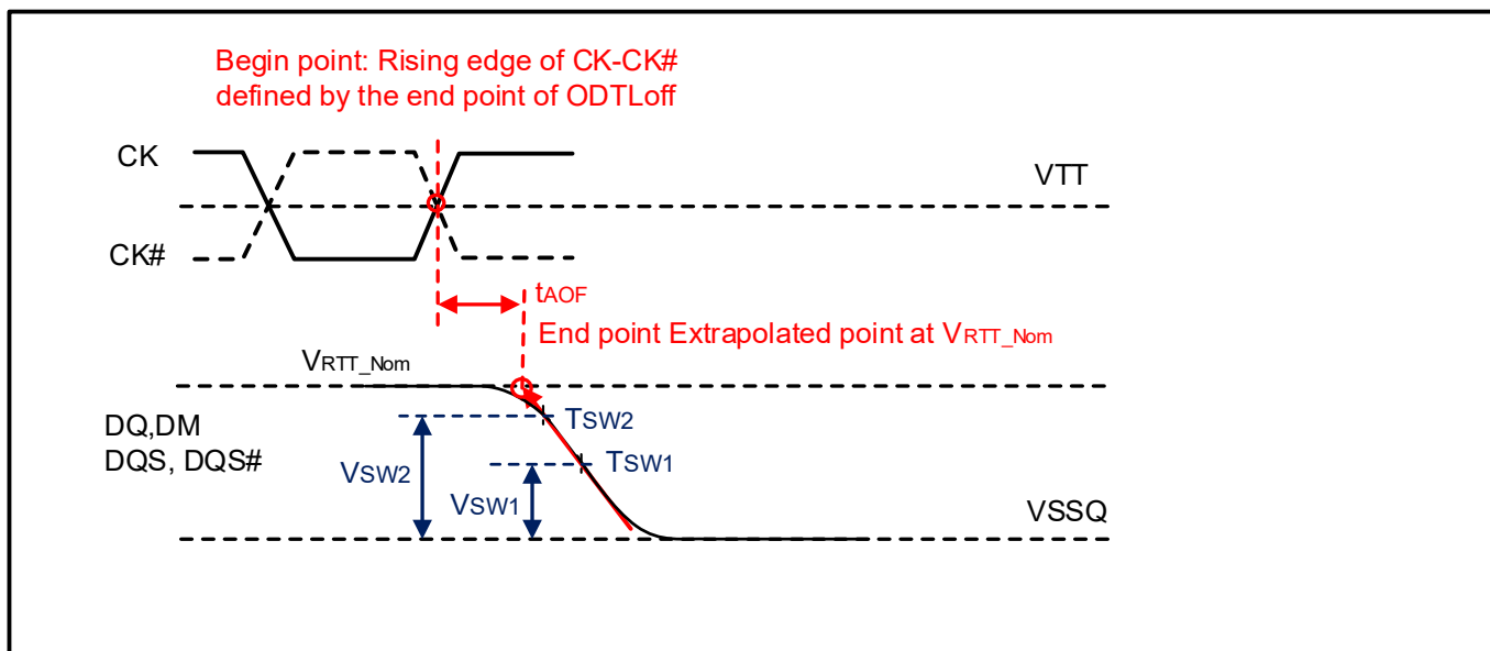
Figure 6-11. Definition of t_{AOF}
