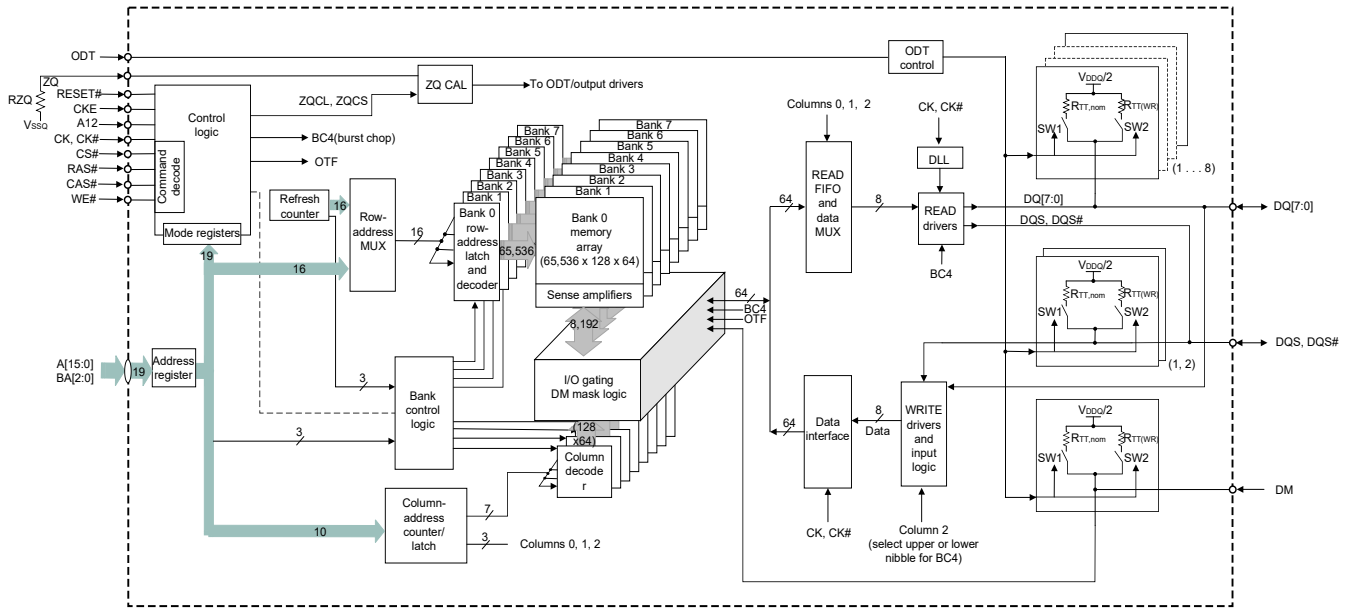
Figure 3-1. 512 Meg x 8 Functional Block Diagram
