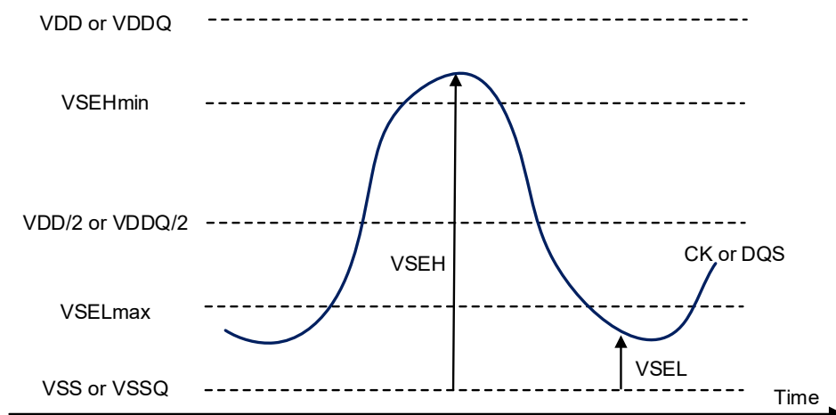
Figure 5-3. Single-ended Requirement for Differential Signals.
