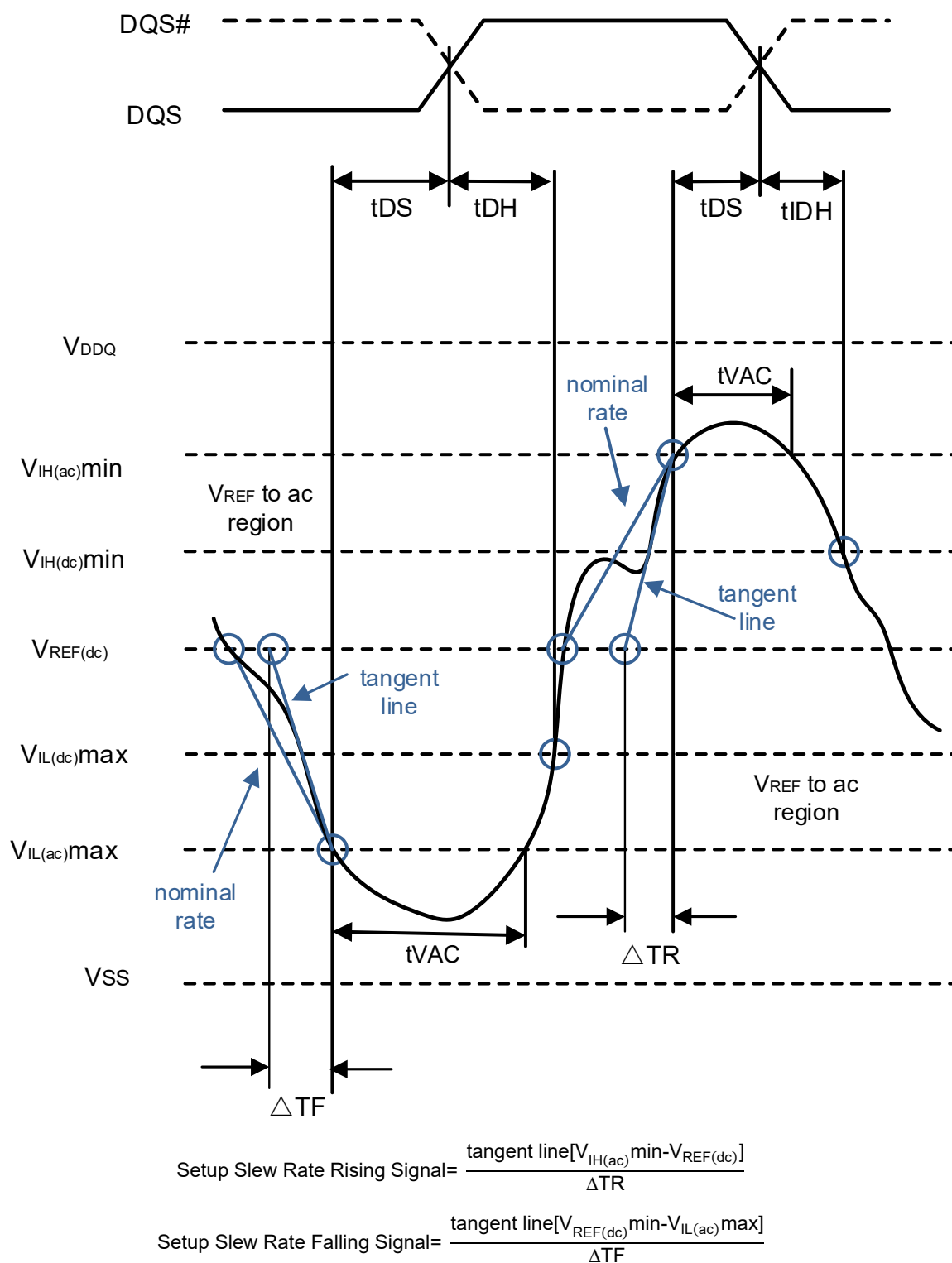
Figure 10-7. Illustration of tangent line for setup time t_{DS} (for DQ with respect to strobe)
