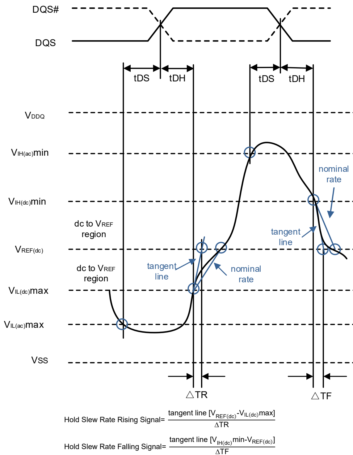
Figure 10-8. Illustration of tangent line for hold time t_{DH} (for DQ with respect to strobe)
