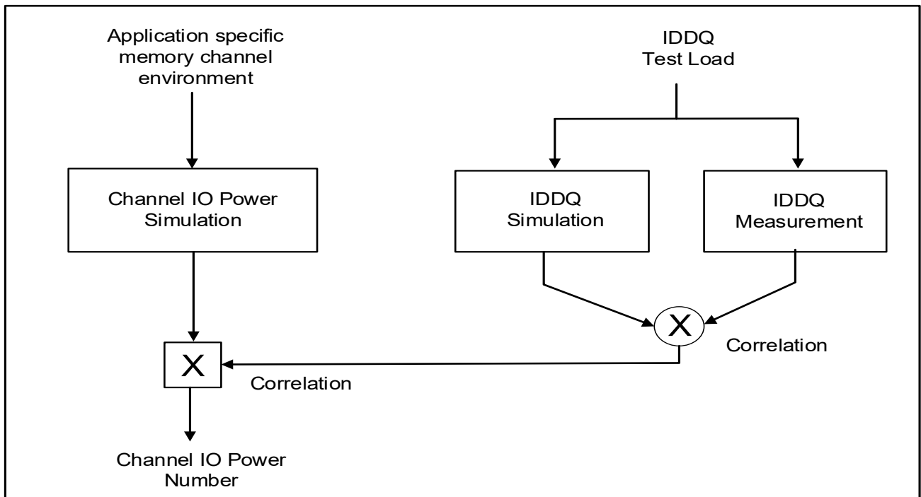
Figure 7-2. Correlation from simulated Channel IO Power to actual Channel IO Power supported by I_{DDQ} Measurement.
