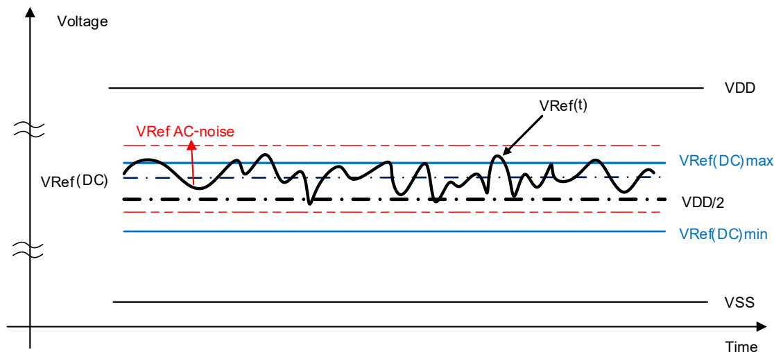
Figure 5-1. Illustration of V_{\text{Ref}}(\text{DC}) tolerance and V_{\text{Ref}} ac-noise limits
