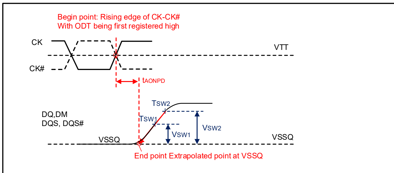
Figure 6-10. Definition of t_{AONPD}
