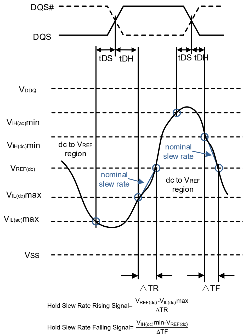
Figure 10-6. Illustration of nominal slew rate for hold time t_{DH} (for DQ with respect to strobe)
