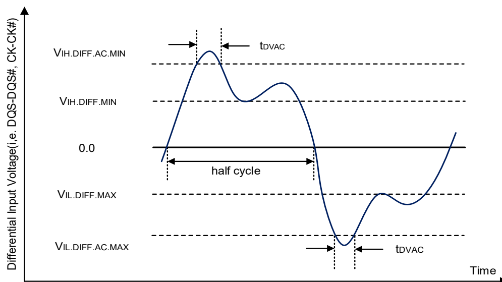
Figure 5-2. Definition of Differential AC-Swing and “Time above AC-Level” t_{DVAC}
