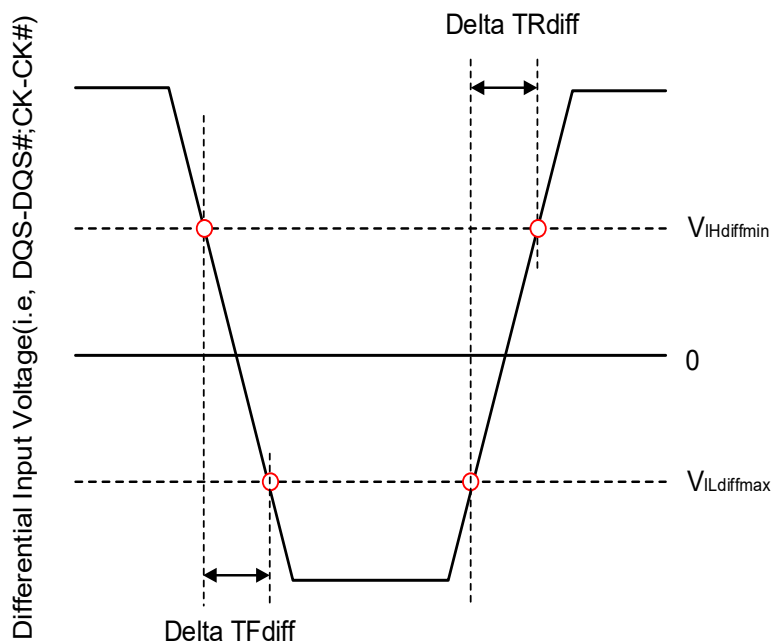
Figure 5-5. Differential Input Slew Rate Definition for DQS, DQS# and CK, CK#
