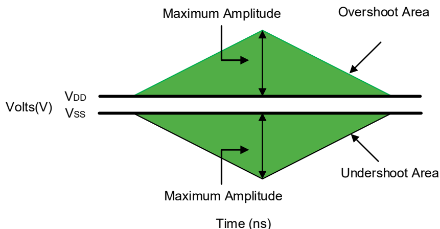
Figure 6-4. Address and Control Overshoot and Undershoot Definition
