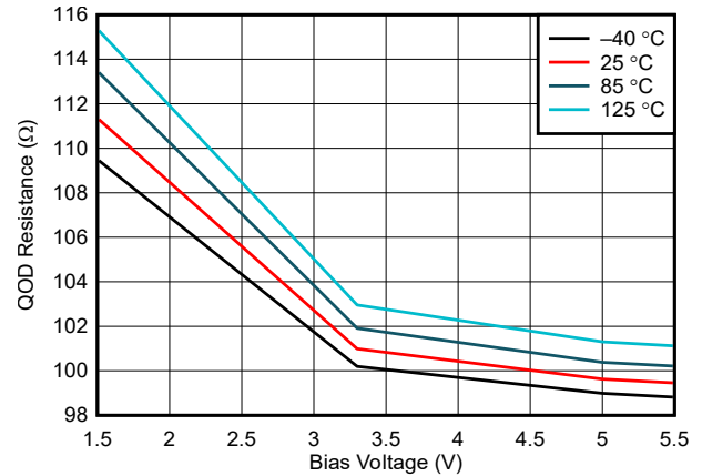
Figure 6-2. QOD Resistance vs Bias Voltage
