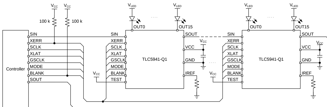
Figure 18. Cascading Devices
