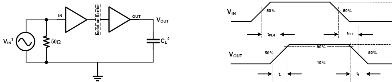
Figure 8. Timing Characteristics Test Circuit and Voltage Wave forms
