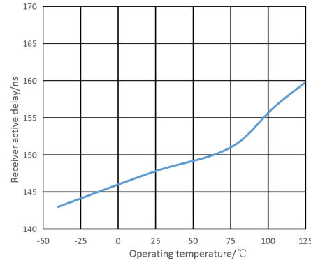
Figure 6. Receiver active delay VS Operating Temperature
