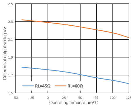
Figure 1. Drive differential output voltage dominant VS Temperature
