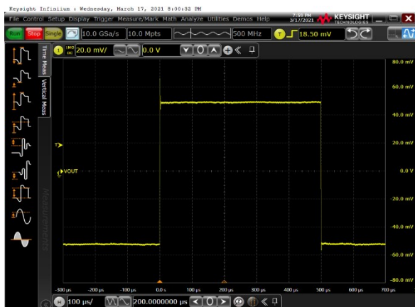
Figure 17. 100-mV Small-Signal Step Response
