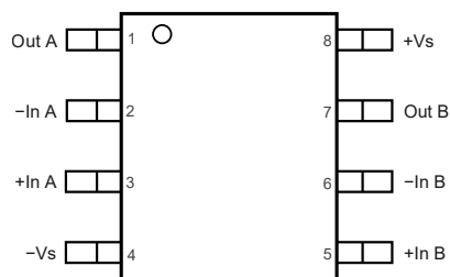
TPA6032 SOP8 Top View
