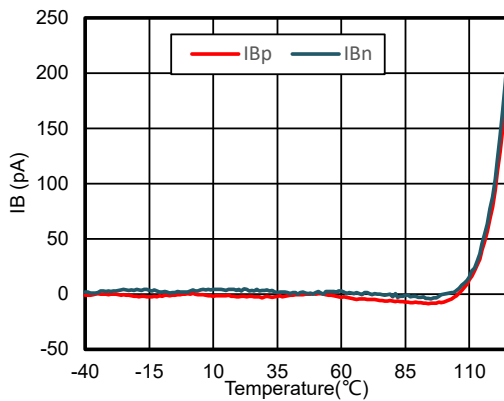
Figure 3. I_B vs. Temperature, -40 to 125°C
