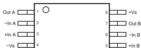
TPA6032 MSOP8 Top View
