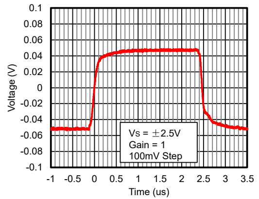
Figure 8. 100-mV Signal Step Response
