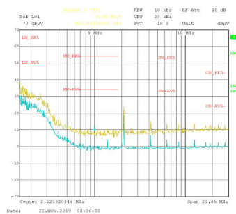
传导 EMI: V_{\text{OUT}} = 5\text{V} , I_{\text{OUT}} = 4\text{A}
