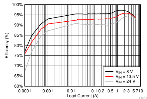
效率: V_{\text{OUT}} = 5\text{V} , F_{\text{SW}} = 400\text{ kHz}
